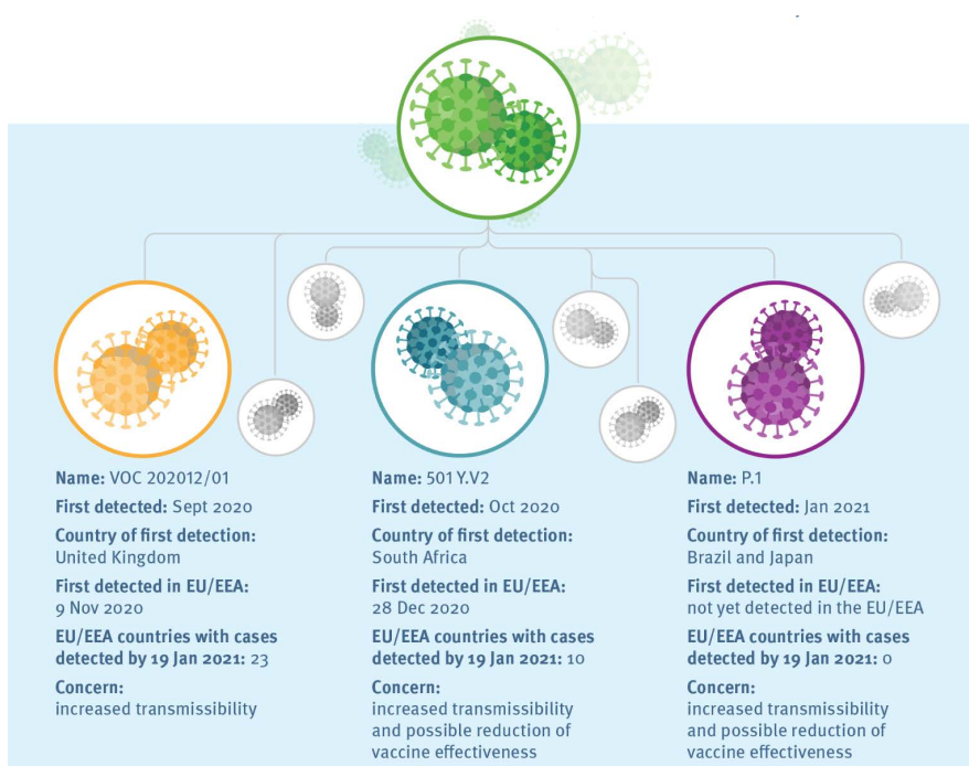
Figure 2. Mutation of SARS-CoV-2. VOC 202012/01: B.1.1.7 – 501Y.V2: B.1.351 . Source and copyright: ECDC Infographics, 21 January.
